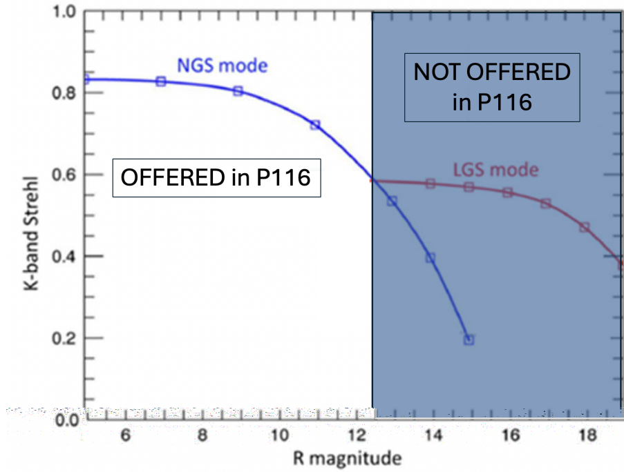
Figure 6: Expected Strehl ratio (SR) in K-band of NGS-VIS in P116 and LGS-VIS (foreseen for P117) modes.
